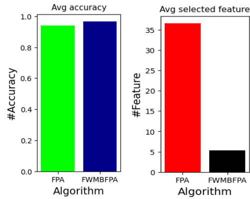
Fig. 2. Average accuracy and selected features obtained by FWMBFPA and BFP.
