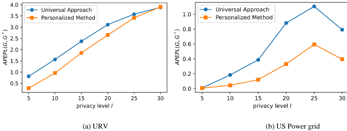
Figure 5. URV dataset and US power grid dataset: APEPL Cost(G, G^*)
